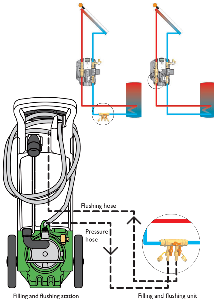
Filling and flushing station
