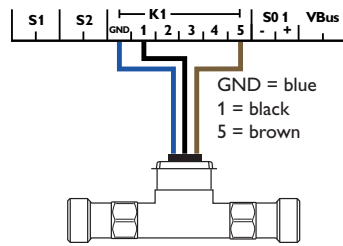
FlowRotor
