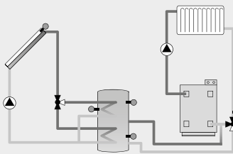
Example 07: Solar system with stratified tank and solid fuel boiler and return flow increase
